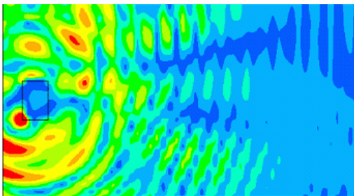
Radiated-field simulation of a telecommunication rack
