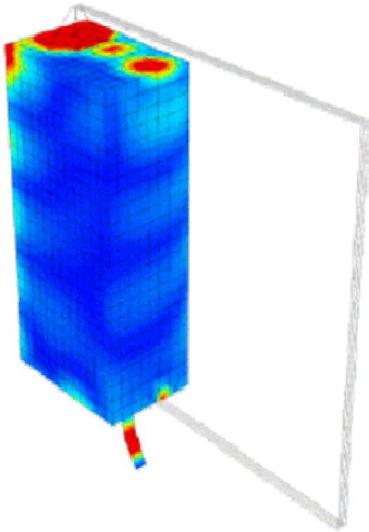
Radiated-field simulation of a telecommunication rack
